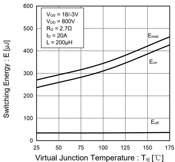
Fig.20 Typical Switching Energy vs. Virtual Junction Temperature
