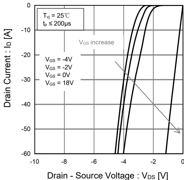
Fig.5 T_{vj} = 25^{\circ}\text{C} 3rd Quadrant Characteristics
