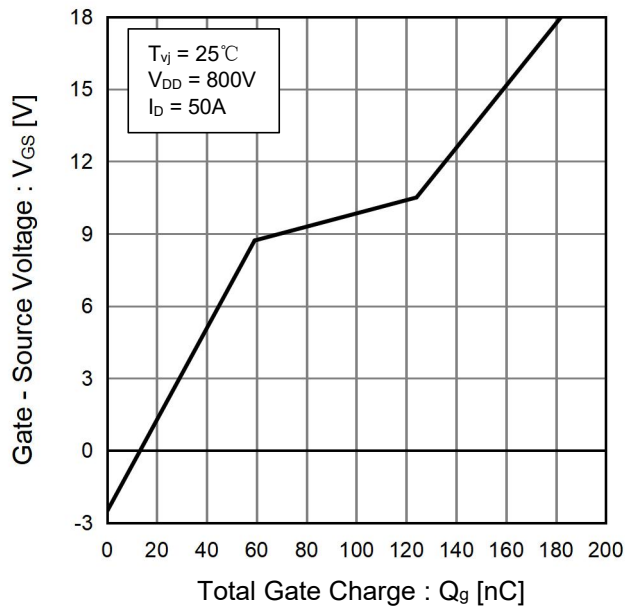
Fig.16 Dynamic Input Characteristics
