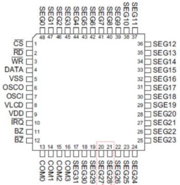
LQFP-48
