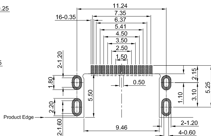
PCB REFERENCE DIAGRAM TOLERANCE:±0.05
