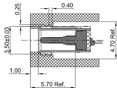
REFERENCE ASSEMBLY
