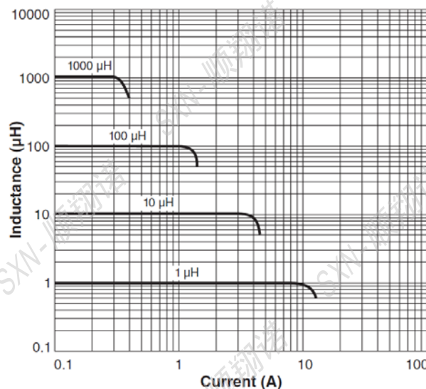
Inductance vs Current
