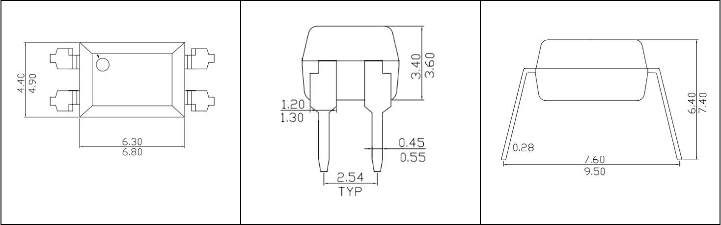
4-pin DIP
