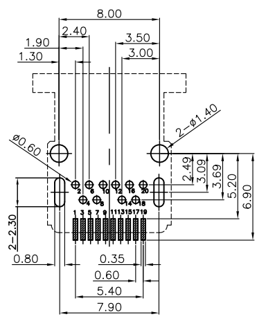
RECOMMENDED PCB LAYOUT TOLERANCE: ±0.05 TOP VIEW
