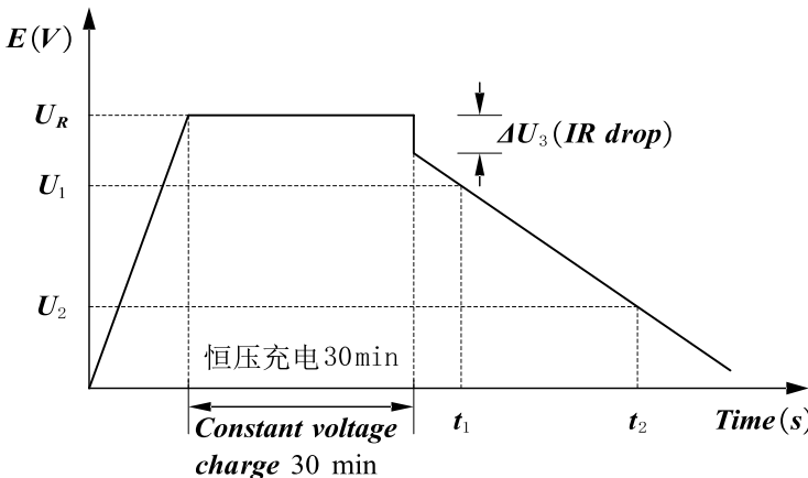
充放电曲线图 / Curve for charge-discharge
