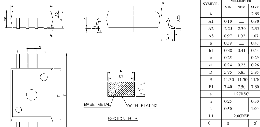
Figure 25. Outline Package
