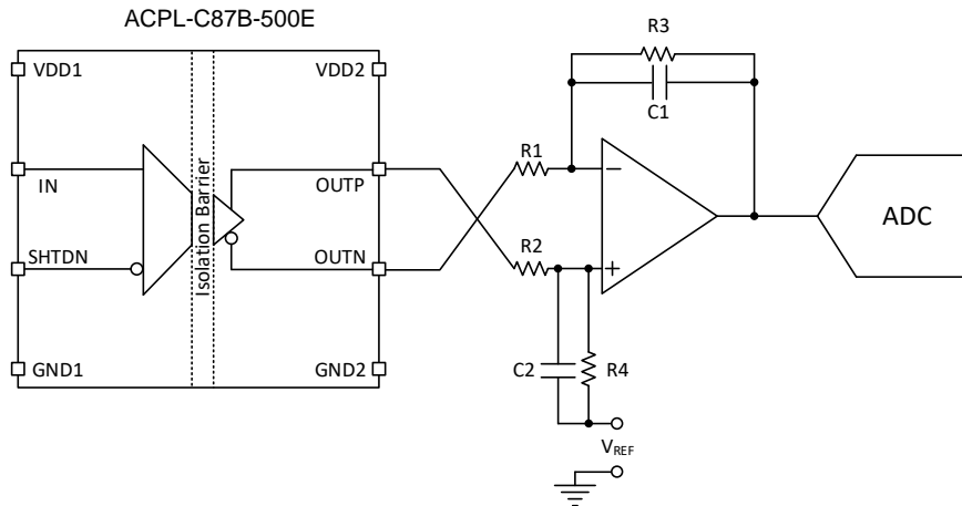
Figure 24. Connecting the ACPL-C87B-500E Output to a Single-Ended Input ADC
