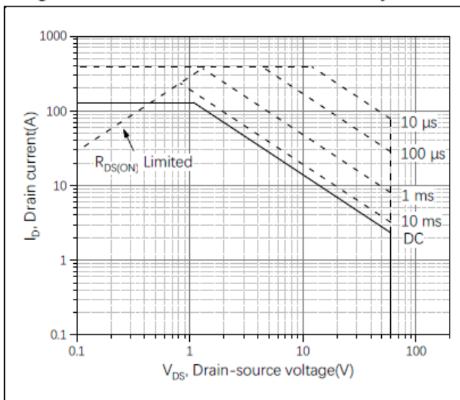
Figure 9, Safe operation area T_C=25\text{ }^{\circ}\text{C}
