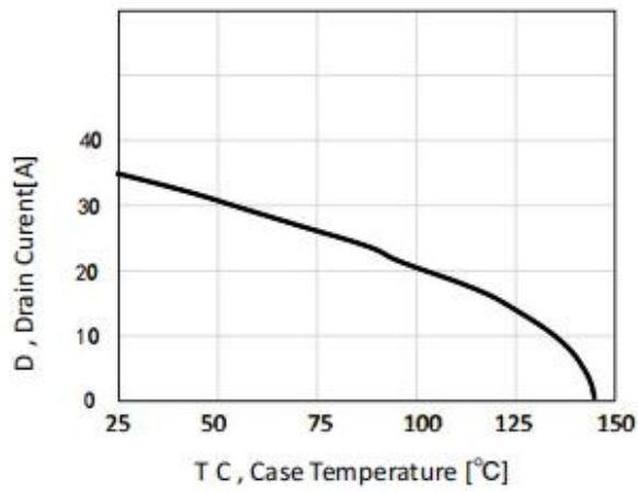
Figure 5. Maximum Drain Current Vs Temperature
