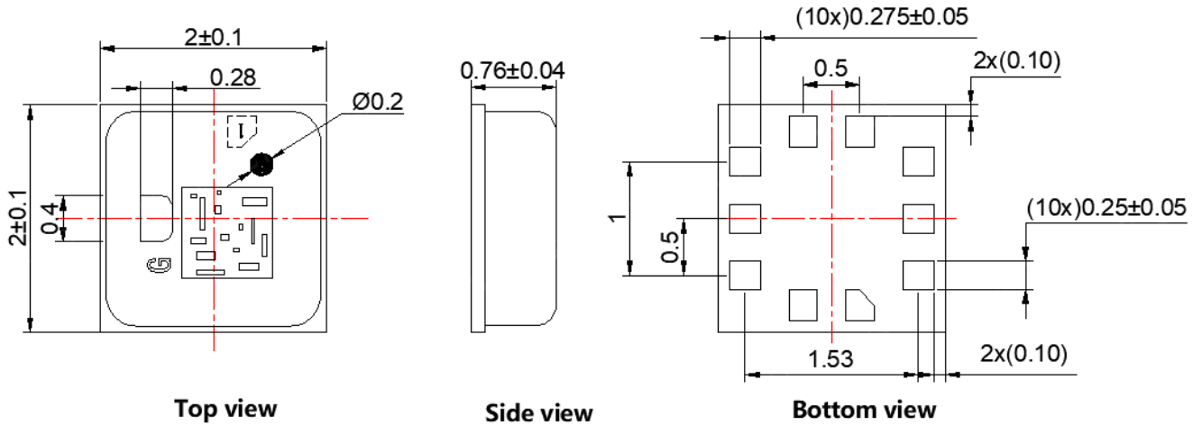
Figure 6: Top view and bottom view of BMP388
