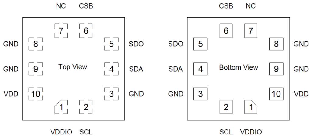
Figure 5: Layout pin configuration BMP388
