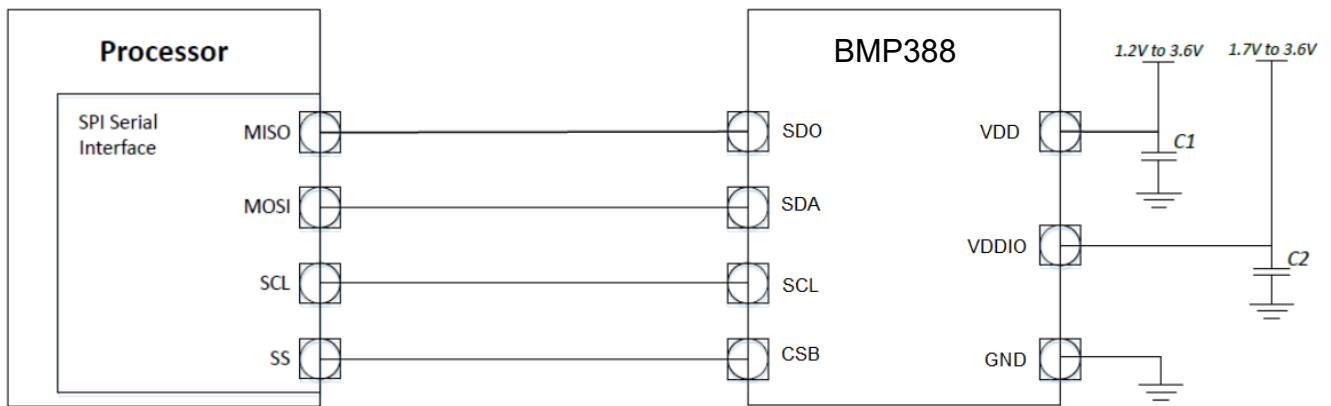
Figure 3: Application circuit example using the SPI 4-wires serial interface
