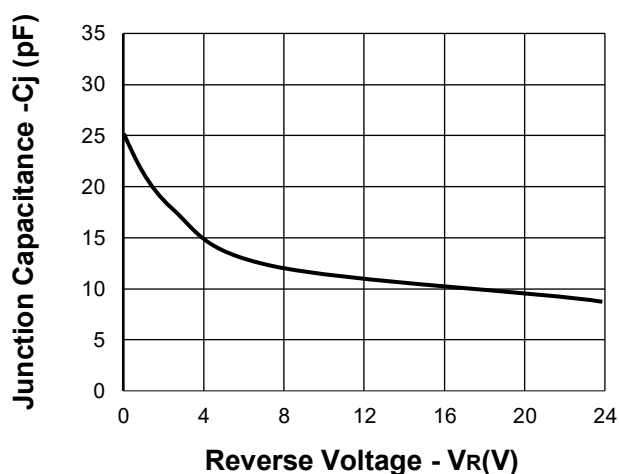
Fig 4. Junction Capacitance vs. Reverse
