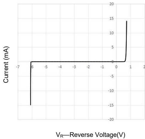
V_R Voltage vs Current
