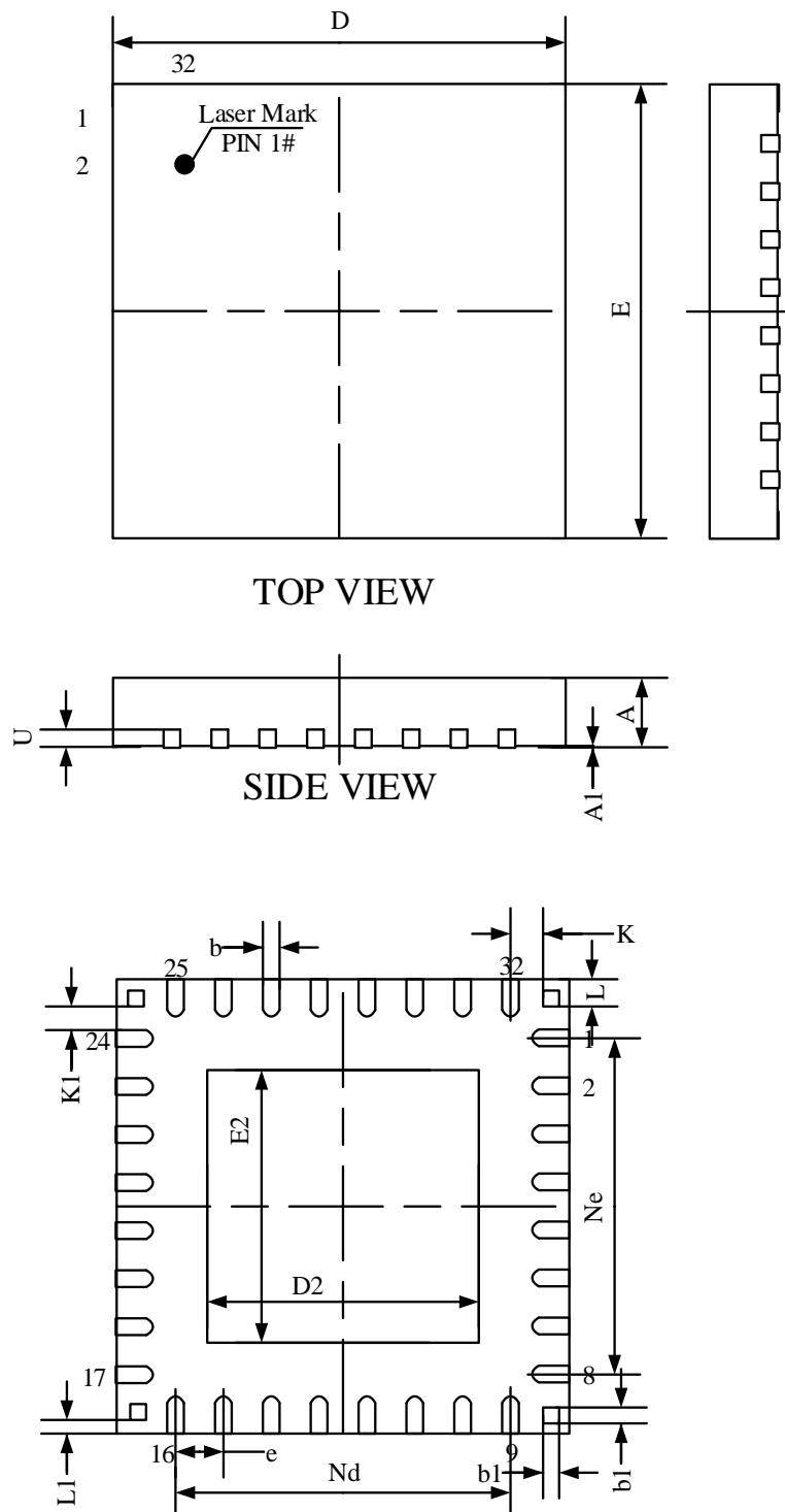
Figure 11-1 Package (QFN32L)
