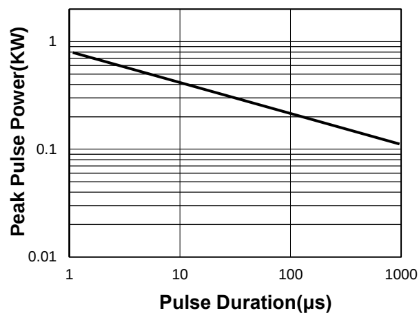
Fig 2. Peak Pulse Power vs. Pulse Time Current
