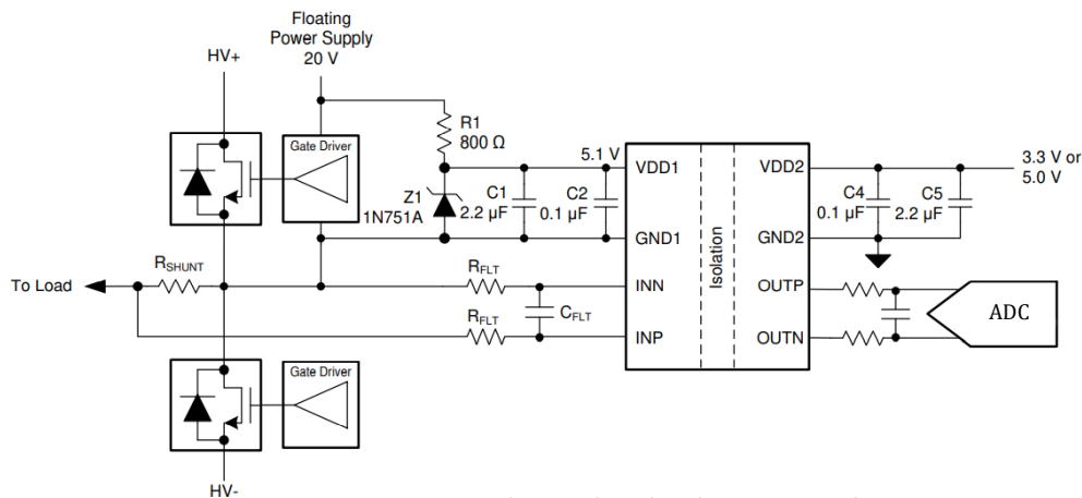
Figure 5. Zener-Diode-Based, High-Side Power Supply
