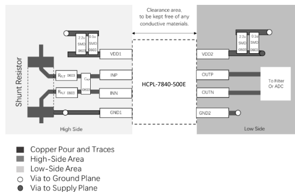
Figure 6. Recommended Layout of the HCPL-7840-500E
