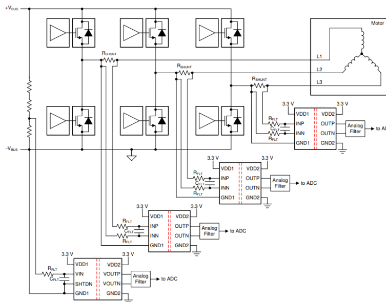
Figure 3. Using the HCPL-7840-500E for Current Sensing in Frequency Inverters
