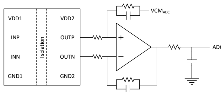
Figure 4. Connecting the HCPL-7840-500E Output to a Single-Ended Input ADC
