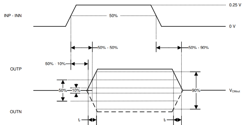
Figure 2. Rise, Fall, and Delay Time Waveforms
