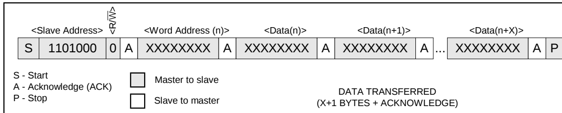
Figure 7. Data Write—Slave Receiver Mode
