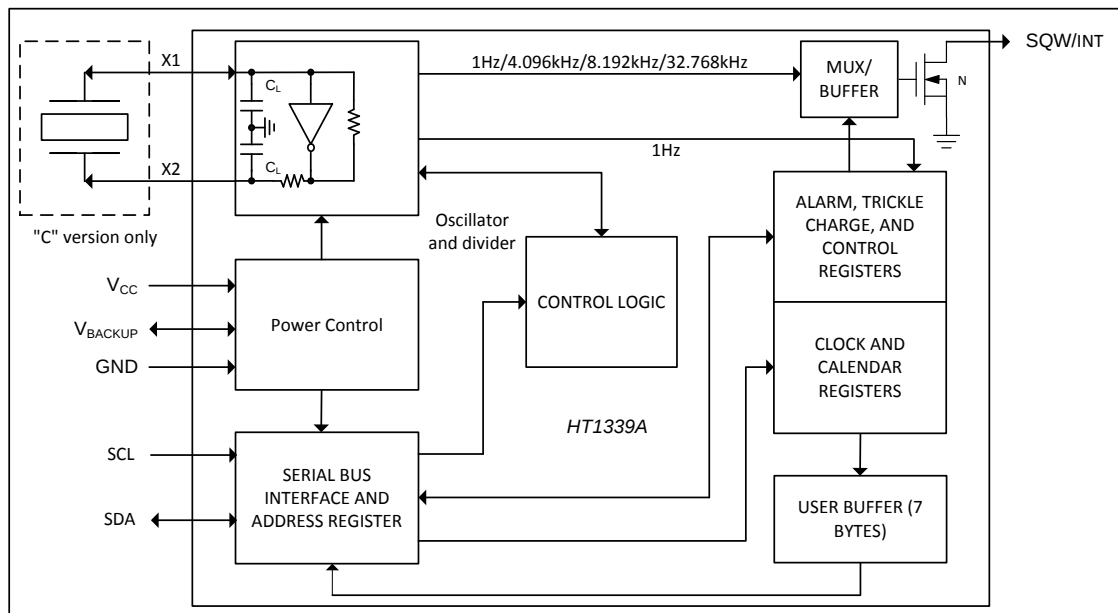
Figure 3. Block Diagram
