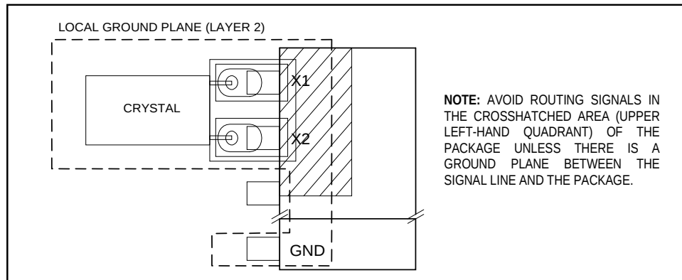
Figure 4. Typical PC Board Layout for Crystal
