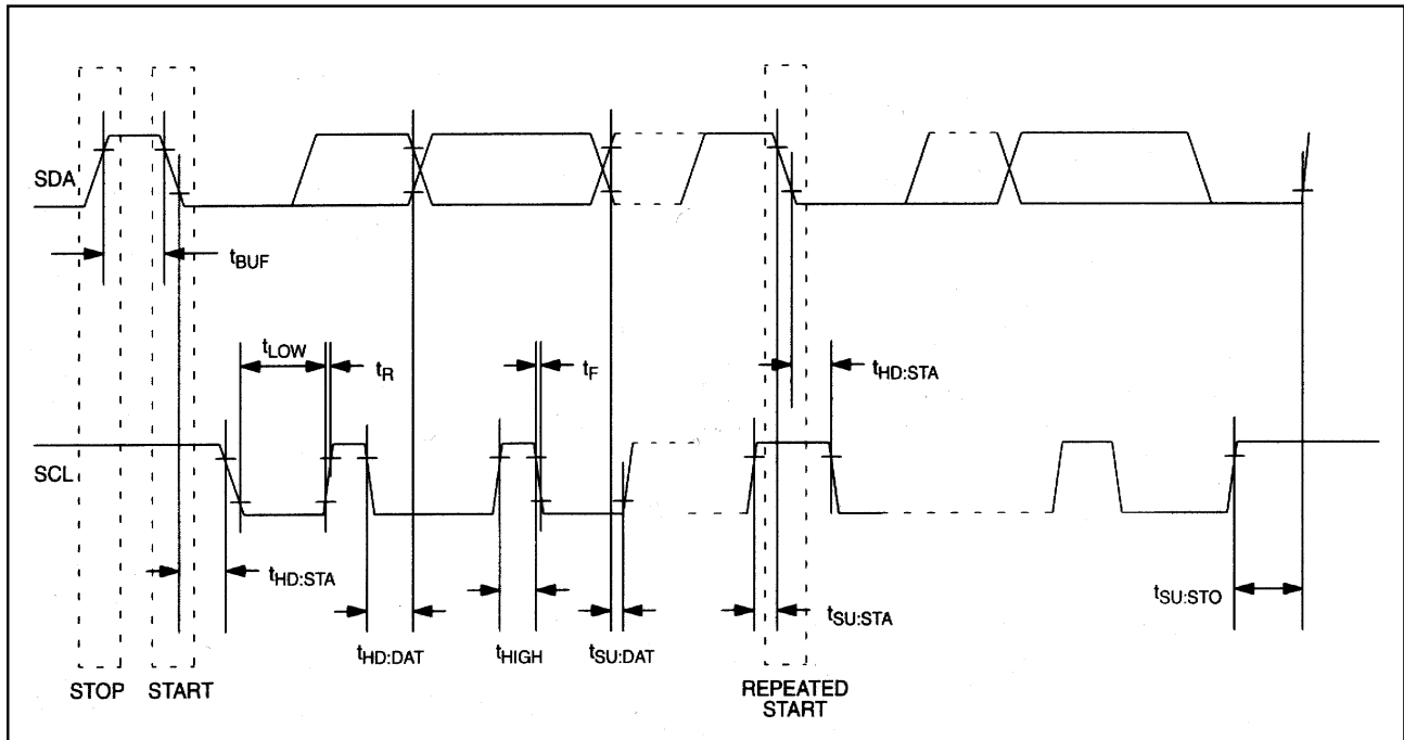
Figure 2. Timing Diagram
