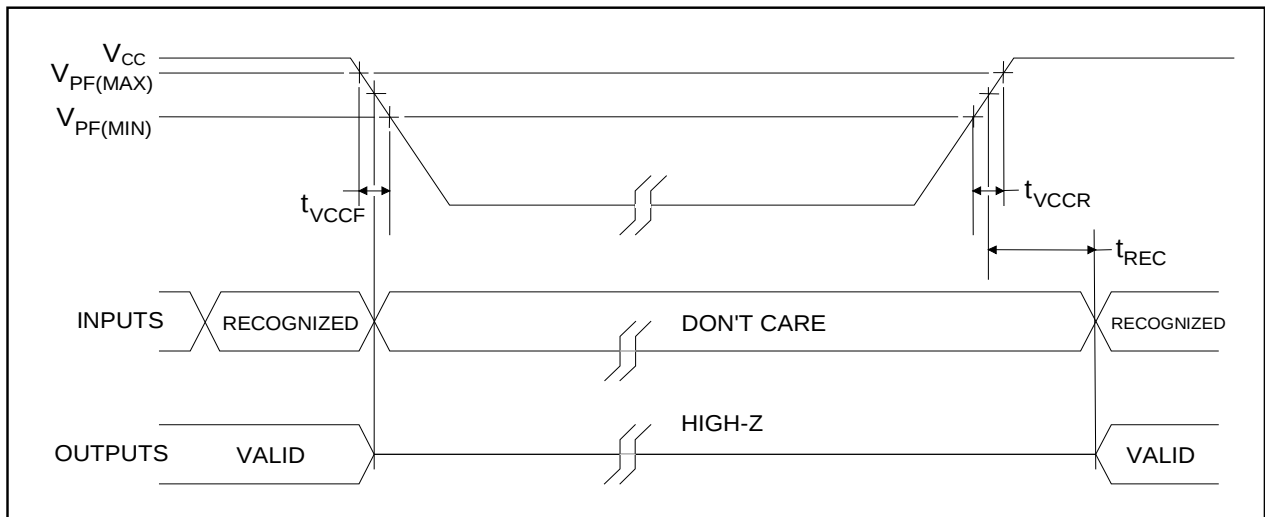
Figure 1. Power-Up/Down Timing
