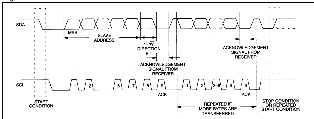
Figure 6. Data Transfer on I 2 C Serial Bus
