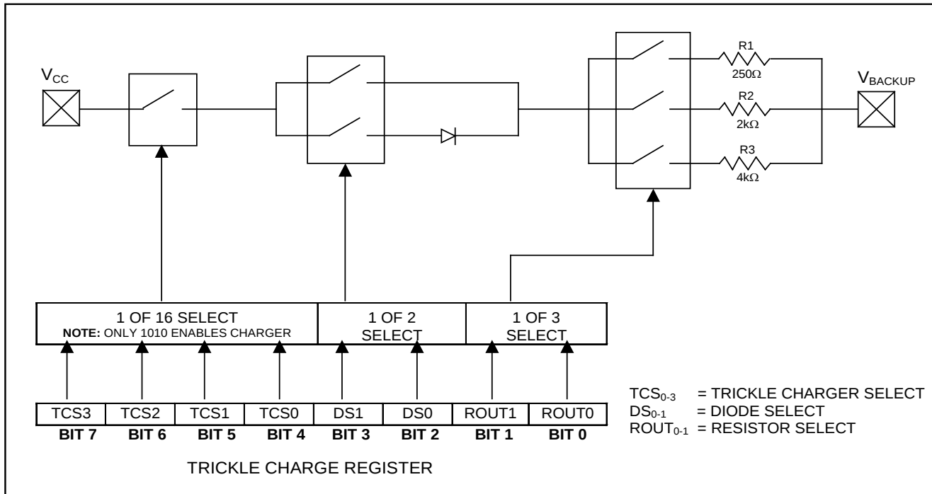
Figure 5. Programmable Trickle Charger
