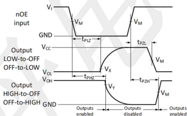
Fig. 5. The input nA to output nY propagation delays
