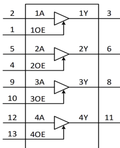
Fig. 1. Logic symbol
