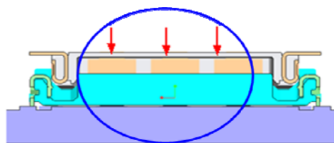
Mating with Parallel(Correct Handling)
