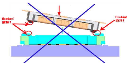
Mating with angle(Wrong Handling)
