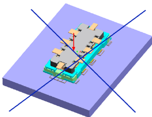
Pushing only Center(Wrong Handling)
