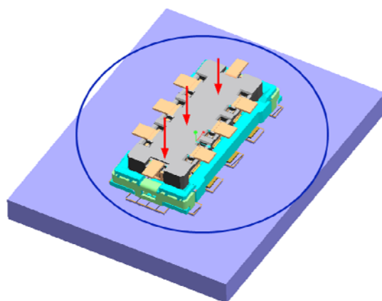
Pushing Whole Paralleled(Correct Handling)
