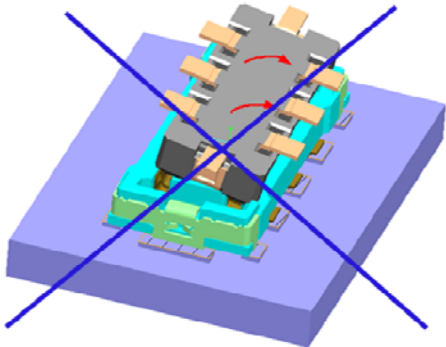
Slant releasing in “b” Direction 短方向的倾斜拔出
