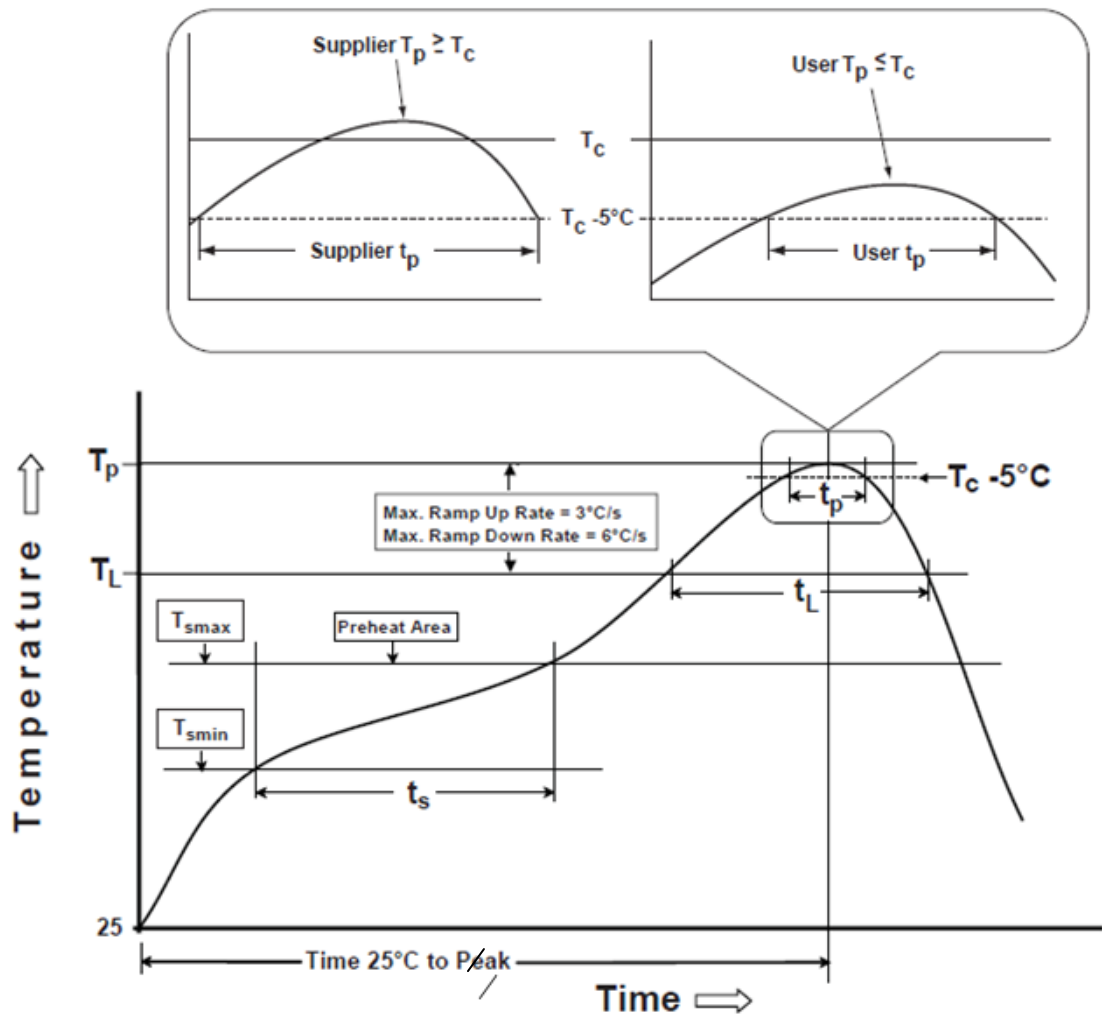
Fig1.Reflow Temperature profile
