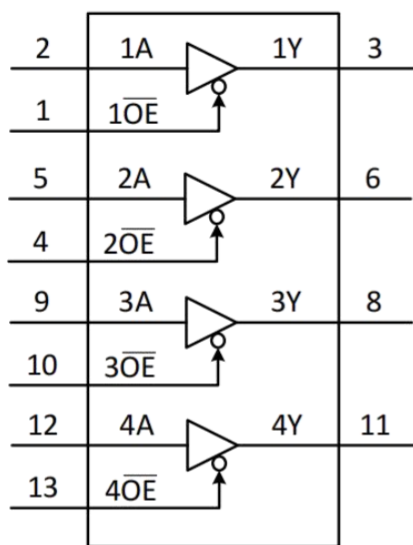
Fig. 1. Logic symbol
