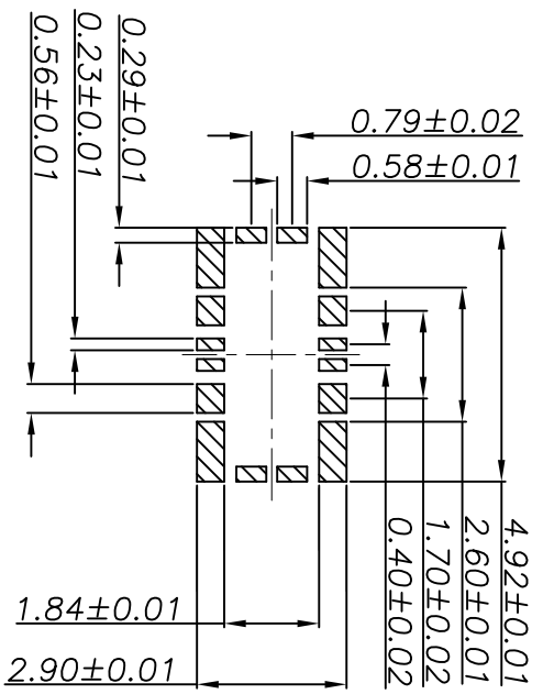
RECOMMEND METAL MASK DIMENSIONS METAL MASK THICKNESS:80um
