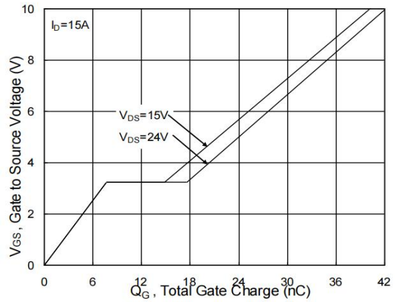
Fig.4 Gate-Charge Characteristics
