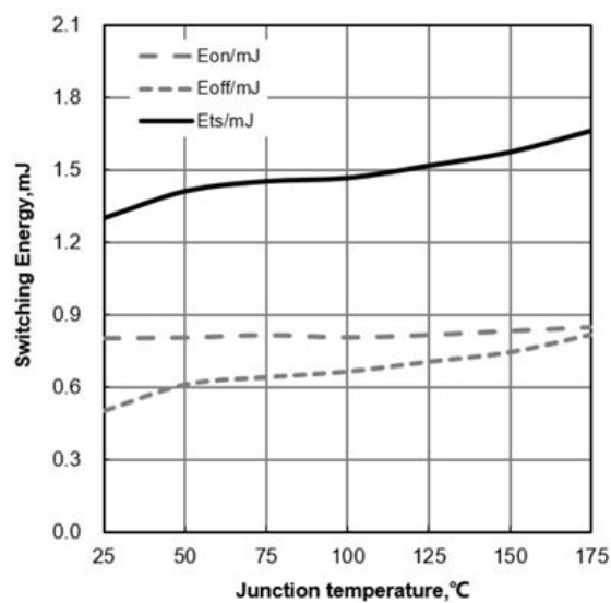
Figure 12. Typical Switching Energy vs Junction Temperature ( V_{CE}=400\text{V} , V_{GE}=15/0\text{V} , I_C=50\text{A} )
