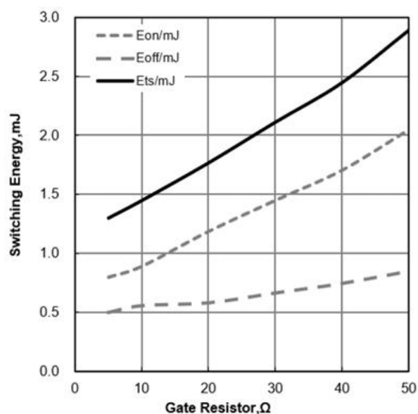
Figure 10. Typical Switching Energy vs Gate Resistor ( T_J=25^{\circ}\text{C} , V_{CE}=400\text{V} , V_{GE}=15/0\text{V} , I_C=50\text{A} )
