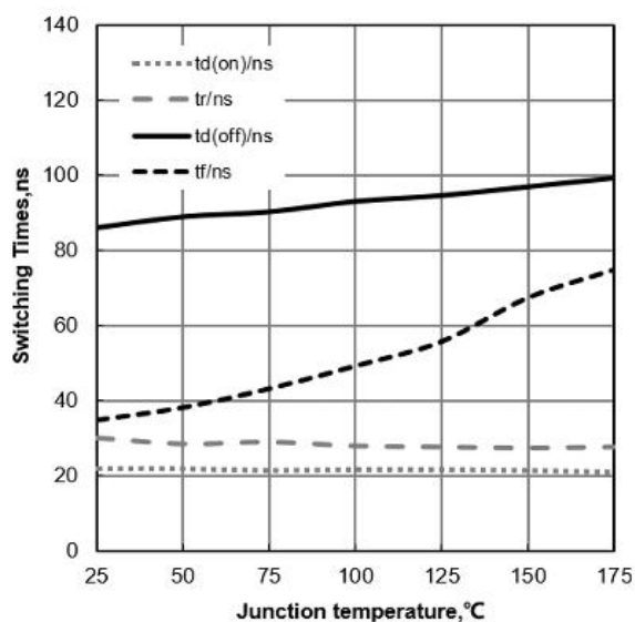
Figure 11. Typical Switching Times vs Junction Temperature ( V_{CE}=400\text{V} , V_{GE}=15/0\text{V} , I_C=50\text{A} )
