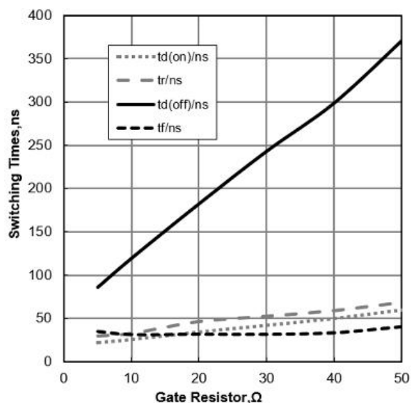
Figure 9. Typical Switching Times vs Gate Resistor ( T_J=25^{\circ}\text{C} , V_{CE}=400\text{V} , V_{GE}=15/0\text{V} , I_C=50\text{A} )
