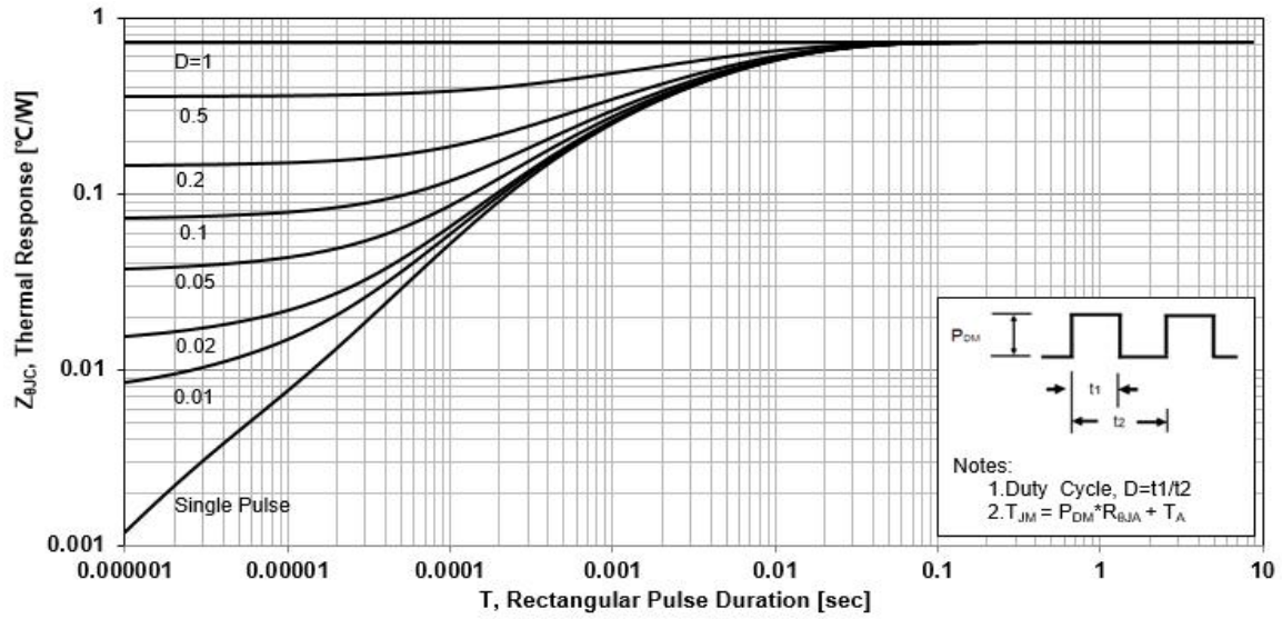
Figure 5. Transient Thermal Impedance
