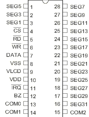
HT1621BNZ DIP28
