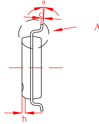
SIDE VIEW 侧视图
