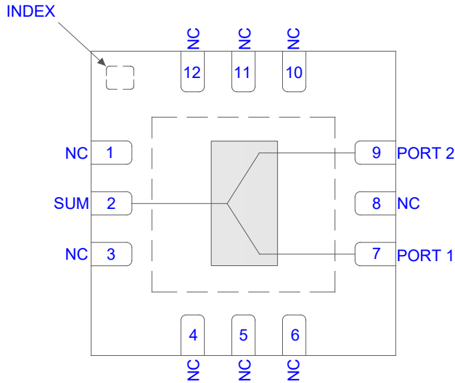
Figure 1. GP2X1A+ Functional Diagram
