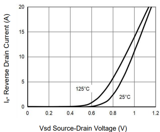
Figure 5. Body-diode characteristics
