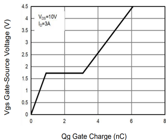
Figure 4. Gate charge
