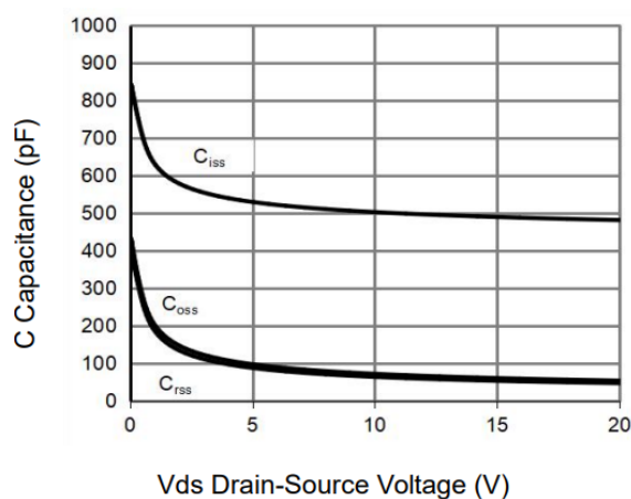
Figure 3. Typ. capacitances
