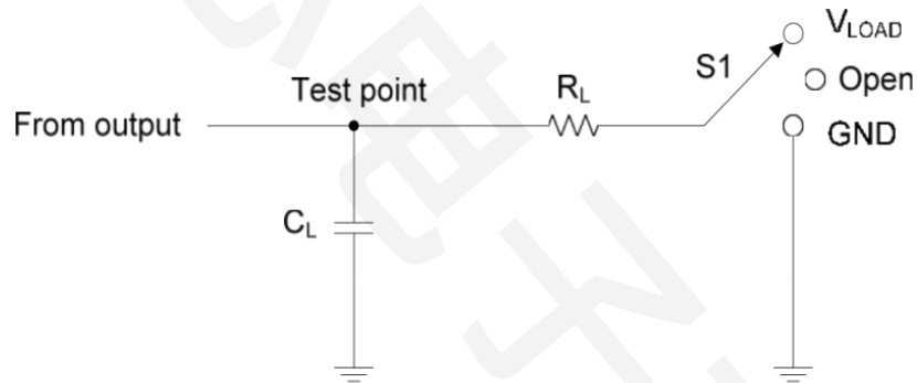
TEST CIRCUIT
