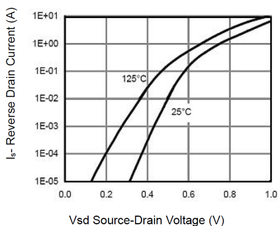
Figure 5. Body-diode characteristics
