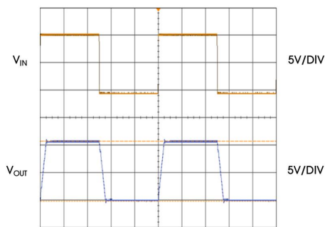
大信号响应 (G = 1)
