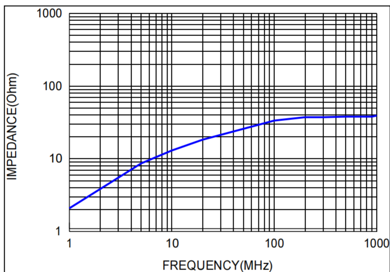
Typical Impedance v.s. Frequency Curve
