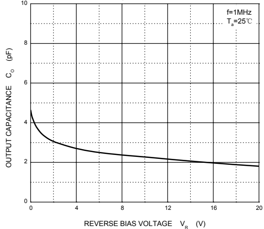
C_O — V_R
