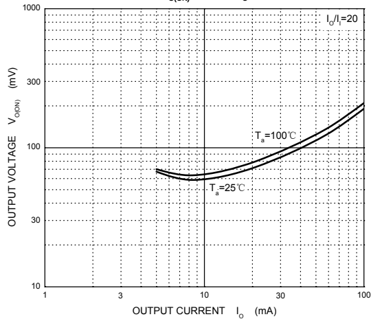
V_{O(ON)} — I_O
