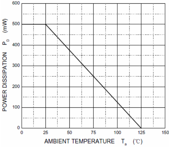
FIG.1-POWER DERATING CURVE
