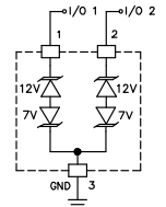
Schematic & PIN Configuration
