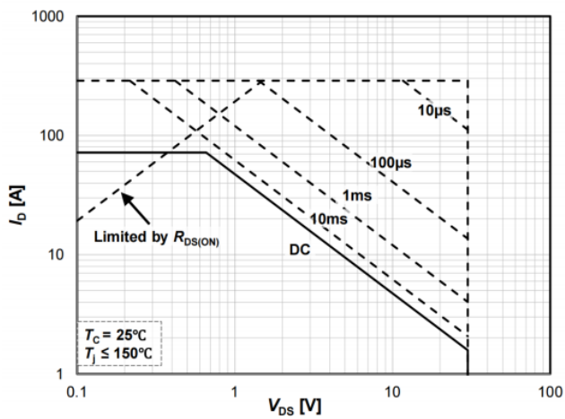
Figure 9. Safe Operating Area 3)
