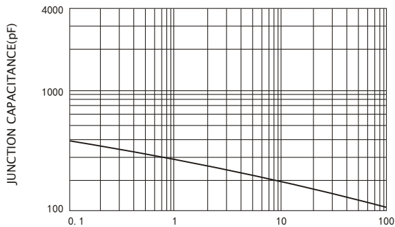
FIG.5-TYPICAL JUNCTION CAPACITANCE
