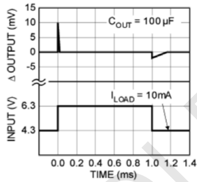
Line Transient.
