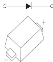
SOD-523
