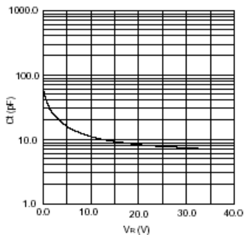
FIG.4-TYPICAL JUNCTION CAPACITANCE
