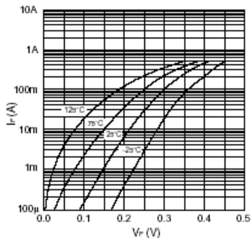
FIG.2-TYPICAL FORWARD CHARACTERISTICS
