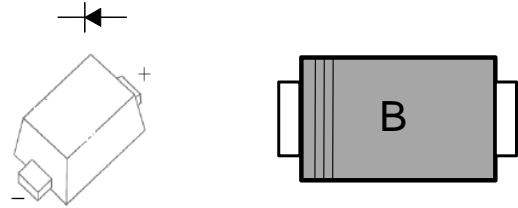
SOD-523
