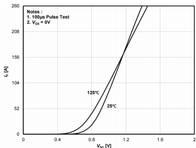
Figure 4. Diode Forward Voltage vs. Current
