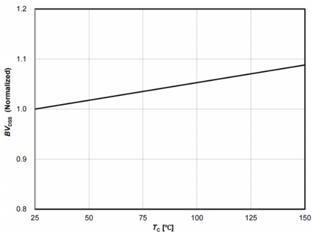
Figure 7. Normalized BV_{DS} vs. Temperature
