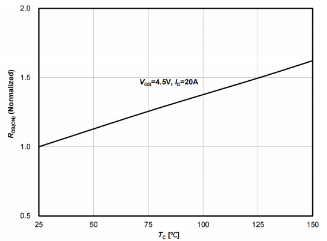
Figure 8. Normalized On-Resistance Variation vs. Temperature
