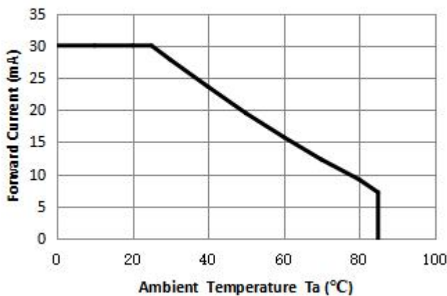
Maximum Forward Current VS. Ambient temperature
