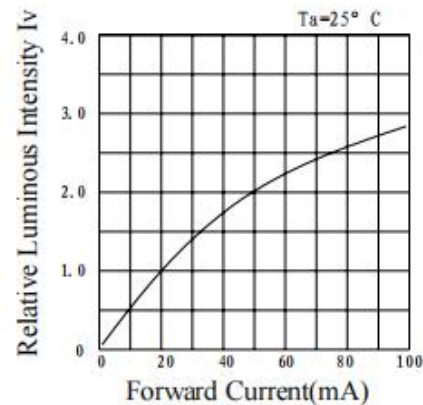
b) 相对光强—正向电流 b) RELATIVE LUMINOUS INTENSITY VS. FORWARD CURRENT
