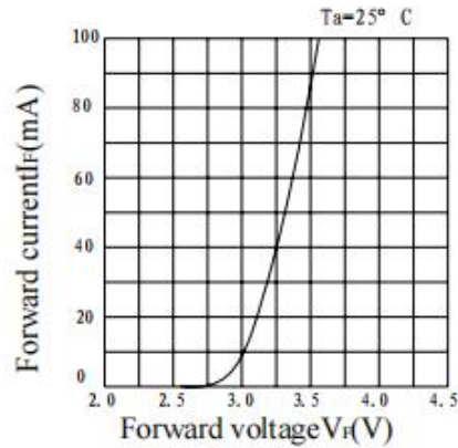
a) 正向电流—正向电压 a) FORWARD CURRENT VS. FORWARD VOLTAGE
