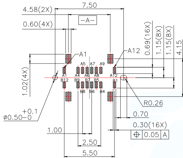
RECOMMENDED PCB LAYOUT(TOP VIEW) THICKNESS 0.8±0.10MM;DEFAULT TOLERANCE:±0.05
