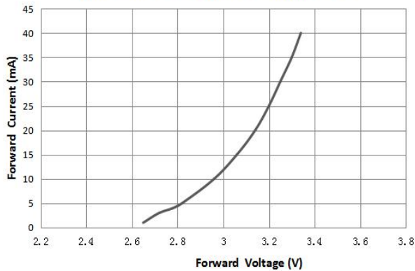
伏安特性曲线 Forward Current VS. Forward Voltage ( T_a=25^\circ\text{C} )
