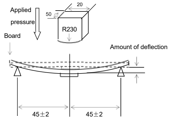
Fig. 4: Bending Strength Test Method
