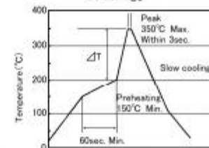
【Recommended condition for Pb-free soldering】
