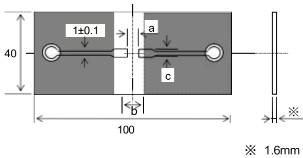
Fig. 3: Board for Bending Strength Test
