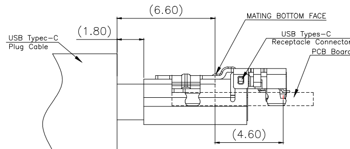
MATED CONDITION SCALE 1:1
