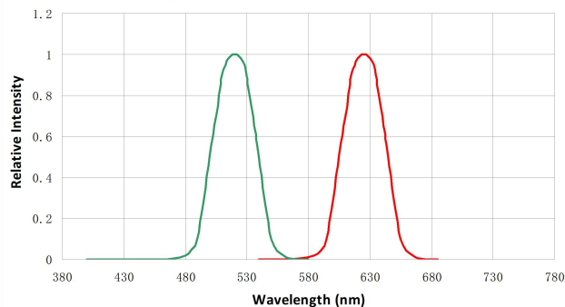
Spectrum Distribution ( T_a=25^\circ\text{C} )
