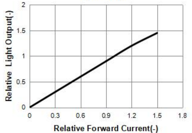
Forward Current VS. light Output ( T_a=25^{\circ}\text{C} )
