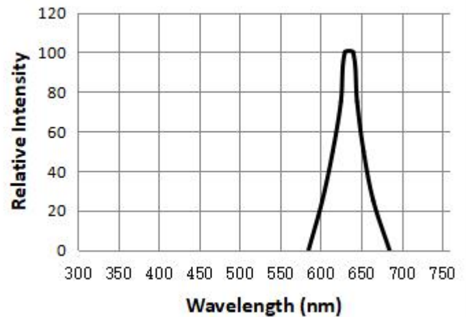
Spectrum Distribution ( T_a=25^{\circ}\text{C} )
